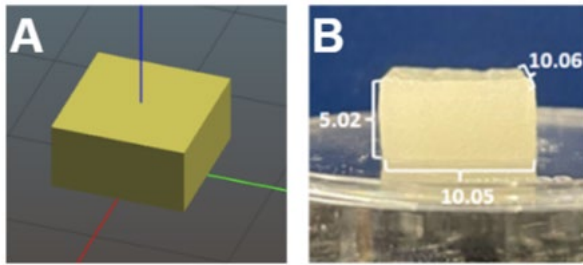
Figure 1. (A) 10x10x5mm CAD model and (B) 3D printed construct after post processing with <math><0.6\%</math> error in printing dimensions.
